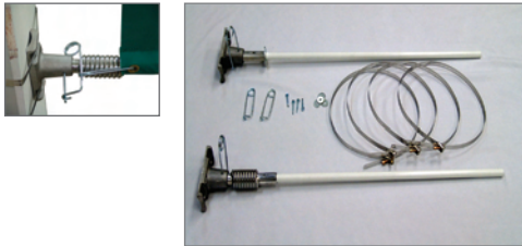
For installations that do not require a Spring Arm Bracket, the Premium Bracket without spring arm offers the same stainless steel sleeve to lengthen the life of the rod. For the longest lasting installations, our premium bracket system is the best choice.
